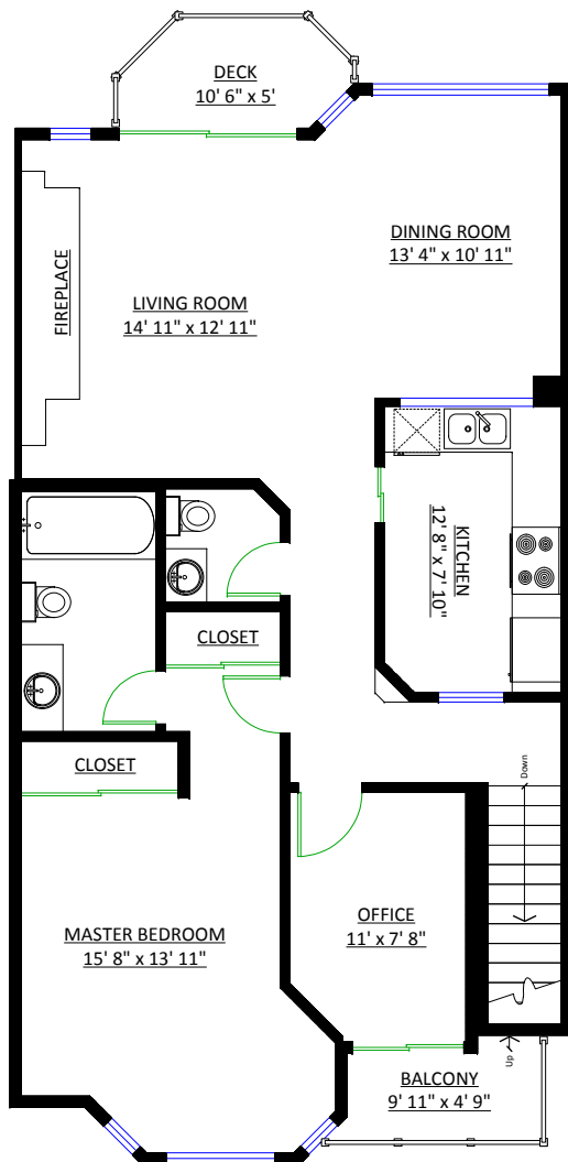
MAIN LEVEL Floor Area: 1,085 Sq. Ft.
